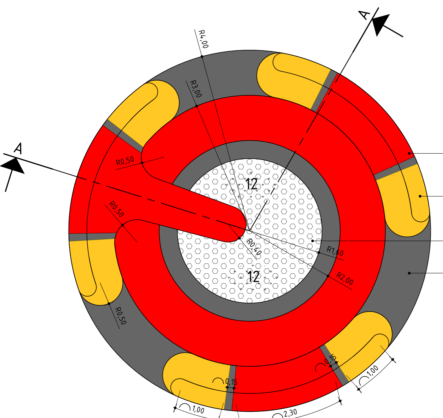
DETAIL A SCHAAAL 1:50
